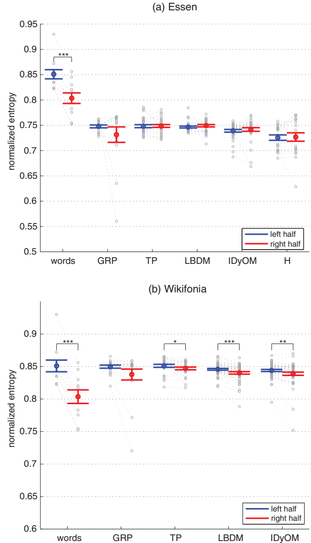
FIGURE 4. Comparison of average normalized entropy of phonemes/scale degrees in the left half and right half of words and musical segments (* p < .05 , ** p < .01 , *** p < .001 ).
